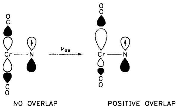
Figure 4. Effect of the asymmetric vibration, \nu_{as} , on the \pi^*-\sigma^* interaction in MLCT-excited \text{Cr}(\text{CO})_4\text{bpy} .
